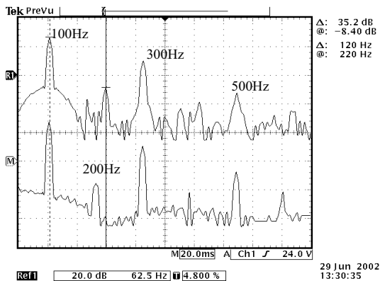
Fig. 9: Spectrum of Unregulated and Regulated Burst Outputs
